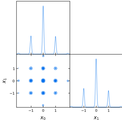
Fig. 3 Rastrigin posterior recovered by MCMC sampling using emcee .
