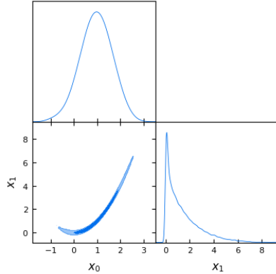
Fig. 1 Rosenbrock posterior recovered by MCMC sampling using emcee .
