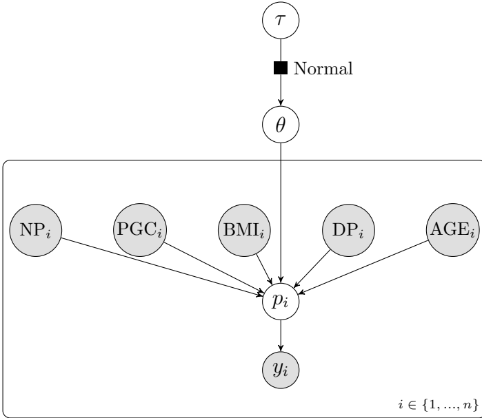
Fig. 7 Graphical representation of logistic regression Model 2 for modelling diabetes in Pima Indians. Model 1 is similar but does not include the AGE covariate.
