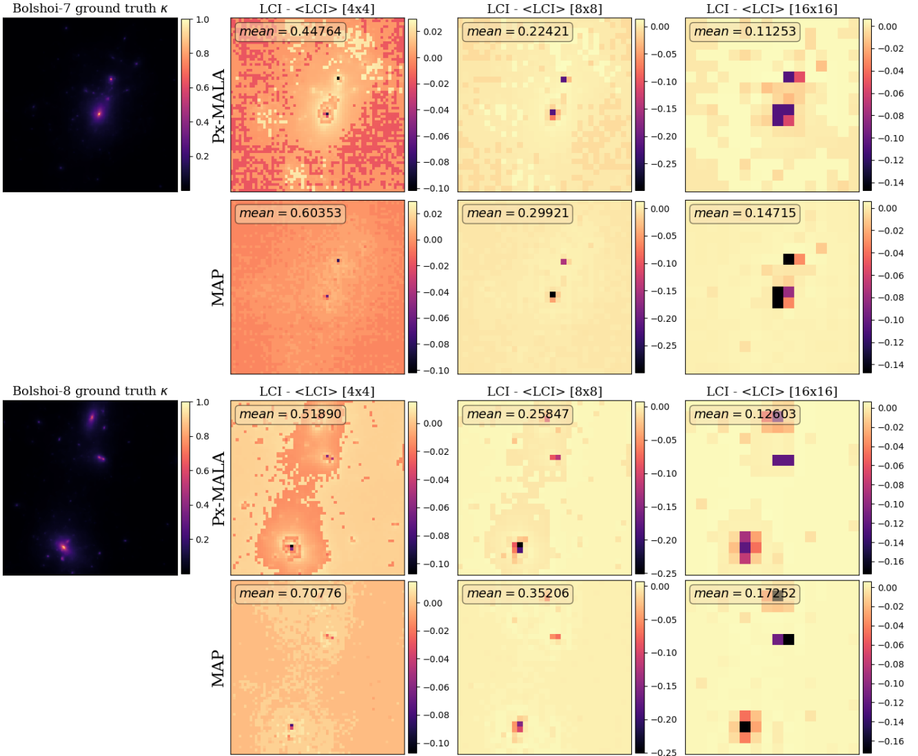
Figure 4. Local Credible Intervals ( cf. Bayesian error bars ) at 99% confidence for the Bolshoi-7 ( top ) and Bolshoi-8 ( bottom ) cluster sparse reconstruction in both the Px-MALA setting ( top ) and MAP ( bottom ) for super-pixel regions of dimension (4 \times 4) , (8 \times 8) , and (16 \times 16) – left to right respectively. Note that these plots display the variation about the mean of each set of LCI’s, with the mean being given numerically in the sub-figure legends – this is done to best display the topological similarity whilst also conveying the absolute difference in size between the methods. Notice that the mean of the MAP LCIs is in all cases larger than that of the corresponding Px-MALA LCIs.
