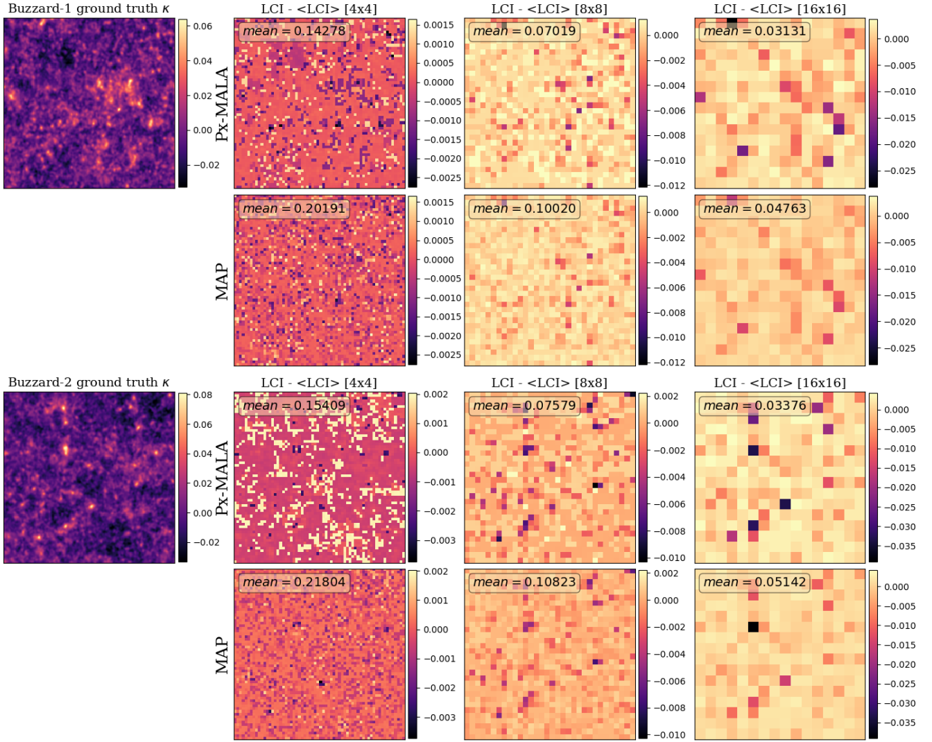
Figure 5. Local Credible Intervals ( cf. Bayesian error bars) at 99% confidence for the Buzzard-1 (top) and Buzzard-2 (bottom) cluster sparse reconstruction in both the Px-MALA setting (top) and MAP (bottom) for super-pixel regions of dimension (4 \times 4) , (8 \times 8) , and (16 \times 16) – left to right respectively. Note that these plots display the variation about the mean of each set of LCI’s, with the mean being given numerically in the sub-figure legends – this is done to best display the topological similarity whilst also conveying the absolute difference in size between the methods. Notice that the mean of the MAP LCIs is in all cases larger than that of the corresponding Px-MALA LCIs.
