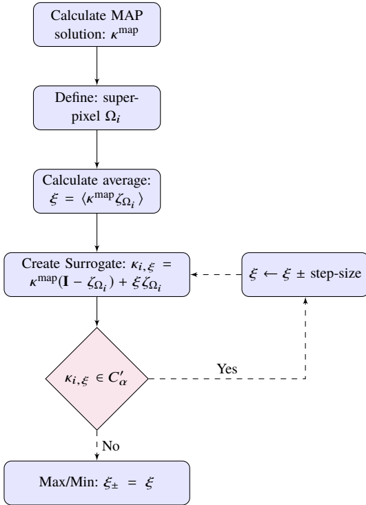
Figure 1. Schematic of the process to construct local credible intervals. At each iterative step the super-pixel region is uniformly increased (decreased) by a step-size. Once the level-set threshold e'_\alpha is saturated the iteration is terminated. Note that this diagram does not represent the bisection method that is adopted in this article, which is a little more involved, but just a simple iterative scheme for conceptualization.
